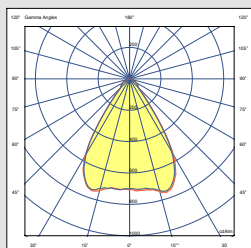
Phenix PC 150W 20110lm 70°
